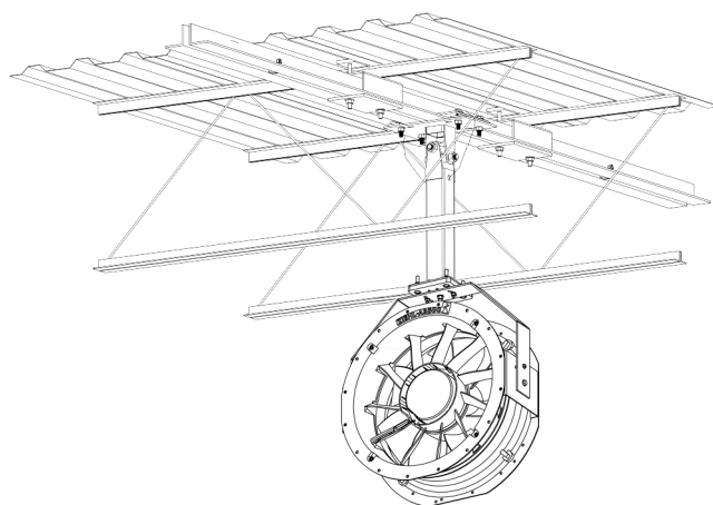
OWSJ MOUNT
